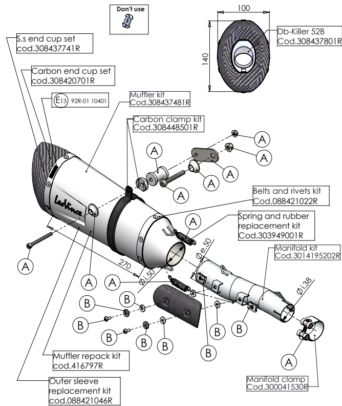
ART. 14195S SPARE PARTS
