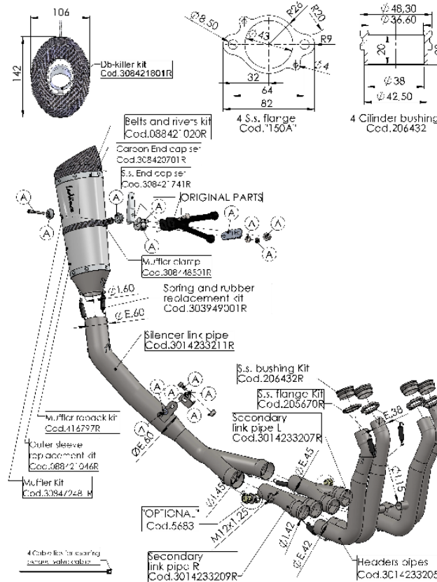
ART. 14233S SPARE PARTS
