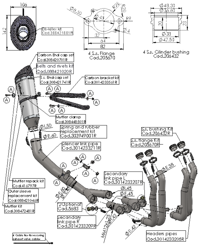
ART. 14233S SPARE PARTS
