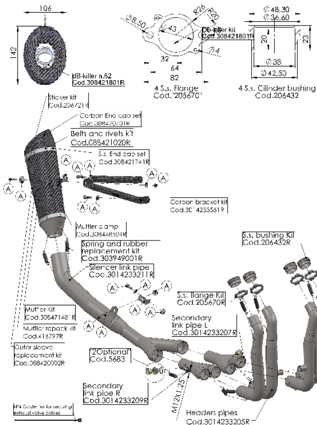
ART. 14234S SPARE PARTS
