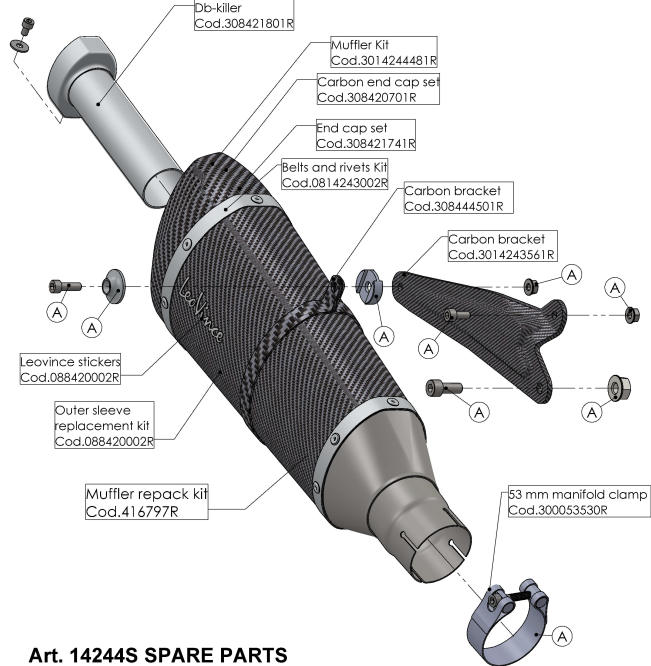
Art. 14244S SPARE PARTS
