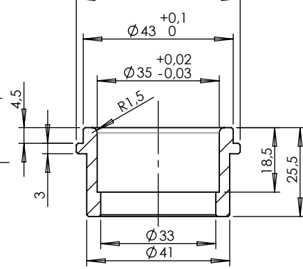
Bushing Cod.204833R
