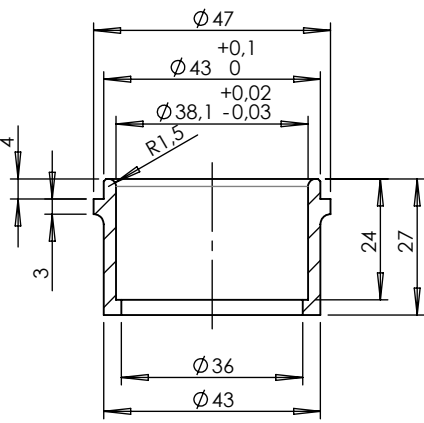
Bushing cod.204870
