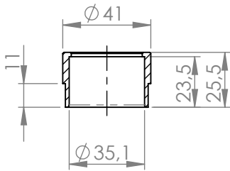
Bushing Cod.206060
