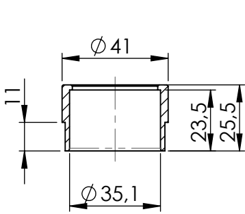
Bushing Cod.206060
