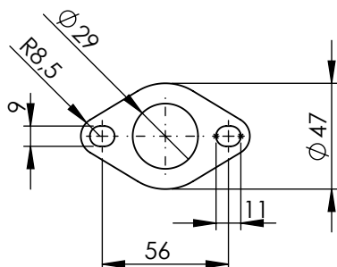
Flange s.s. sp.6mm "45B" cod.204392
