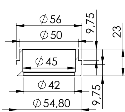
bushing cod.206424
