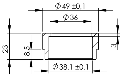
Bushing s.s. cod.207015R
