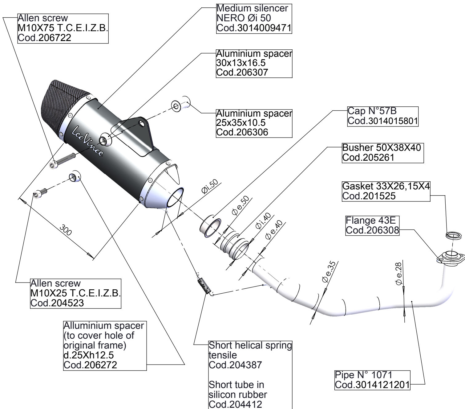
Flange 43E (Th.5)
