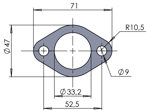
Flange 43E (Th.5)
