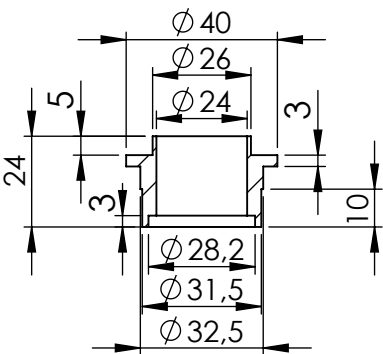
Bushing s.s. cod.204640
